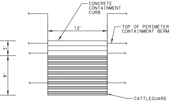
EXIT CATTLEGUARD AND CONTAINMENT CURB (PLAN VIEW) N. T. S.
